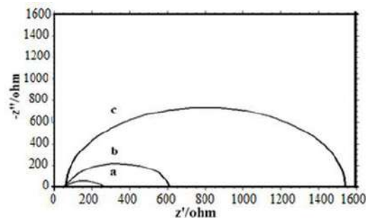
Figure.10: Electrochemical Impedance spectra of a) GO b) P-NMPy and c) GO/P-NMPy
