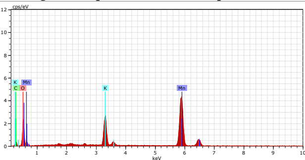
Fig 5: EDAX image of MnO nanoparticle
