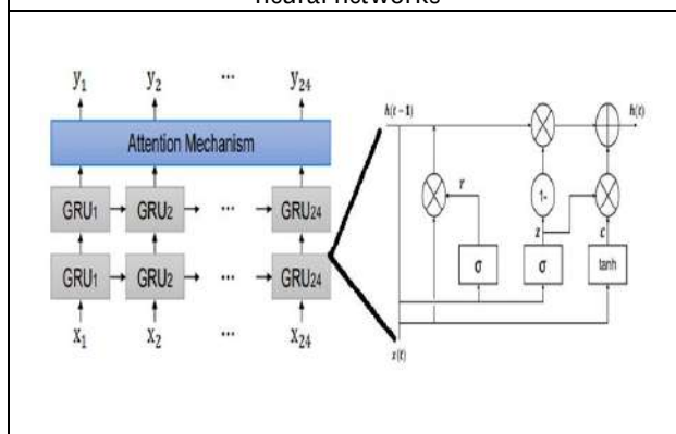
Figure.3: Architecture of Attention Based GRU Model
