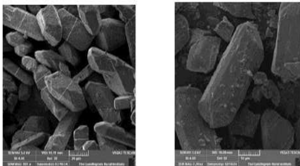
Figure.5: SEM analysis of Cu Nanoparticles
