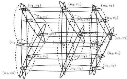
Figure.7: Cartesian Product of Two Semihypergraphs
