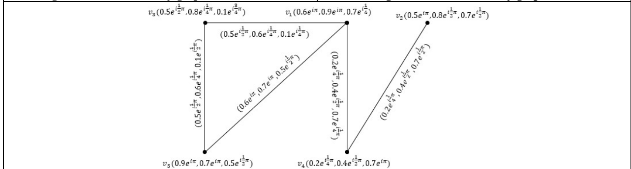
Figure 11: Cohesive fuzzy graph of \bar{G}
