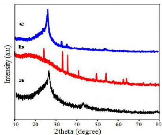
Figure.4: XRD spectrum of a) GO b) P-NMPy and c) GO/P-NMPy polymer composite.
