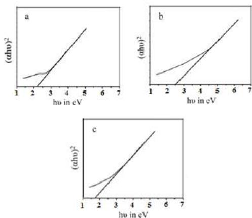
Figure.3: Band gap of a) GO b) P-NMPy and c) GO/P-NMPy polymer composite.
