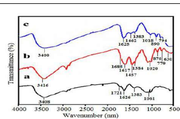
Figure.1: FTIR spectrum of a) GO b) P-NMPy and c) GO/P-NMPy polymer composite.
