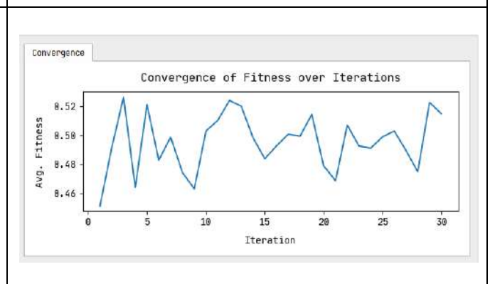
Figure.4: Convergence of fitness over Iterations
