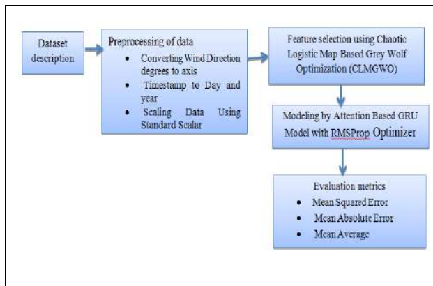
Figure.1: Block diagram for weather forecasting using neural networks
