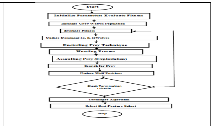
Figure.2: Flow diagram for Feature selection using CLMGWO
