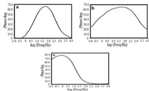
Figure.9:Bode plot of -phase angle/ deg. versus log (f/Hz) for a) GO b) P-NMPy and c) GO/P-NMPy polymer composite
