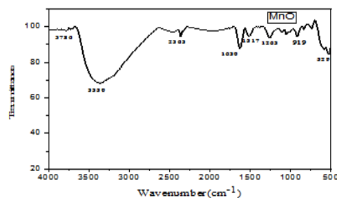
Fig:2 FT-IR Spectrum of MnO nanoparticles
