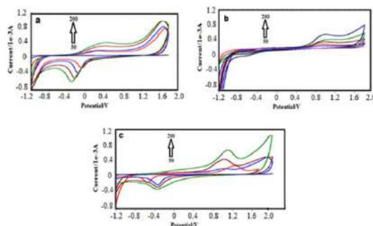
Figure.8:Cyclic Voltammetric behavior of a) GO b) P-NMPy and c) GO/P-NMPy polymer composite
