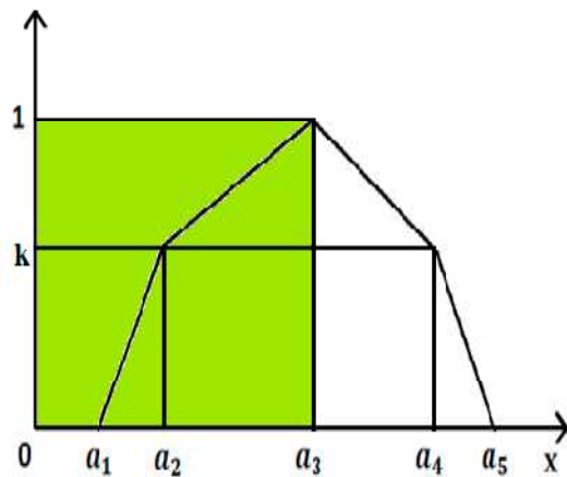
Figure 4.Third step for the RA method
