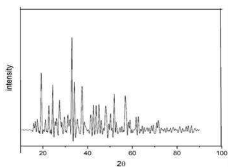
Figure.7: XRD analysis of Cu nanoparticles
