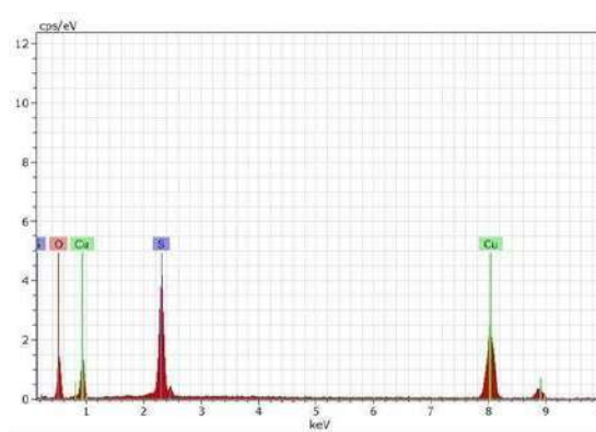
Figure.6: EDX analysis of Cu nanoparticles
