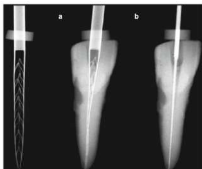
Figure. 5 A to B: (A) The compressibility and adaptability of SAF#20; (B) The conformation of the SAF vs rotary instrumentation
