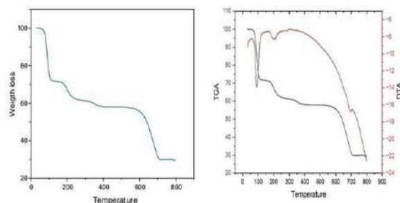
Figure.8: TGA and DTA analysis of Cu Nanoparticles
