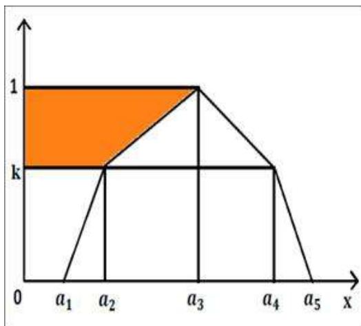
Figure 3.Second step for the RA method
