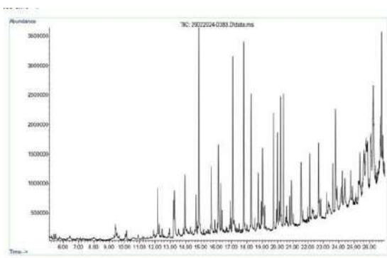
Figure.9: GC-MS analysis of areca fiber extract
