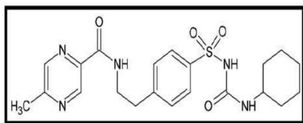
Figure.1: Glipizide structure
